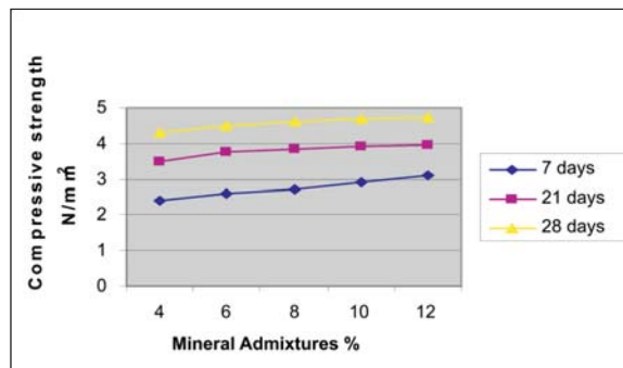
Fig. 2. Cylinder Compressive strength N/mm 2
