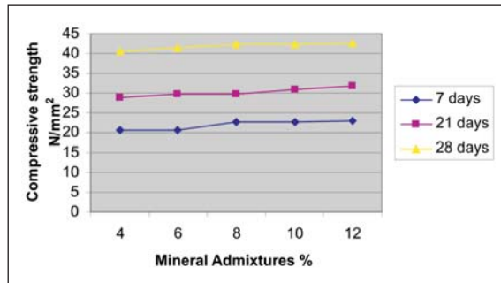
Fig. 1. Cube Compressive strength N/mm 2
